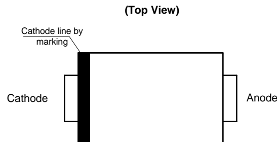
DO-214AC
