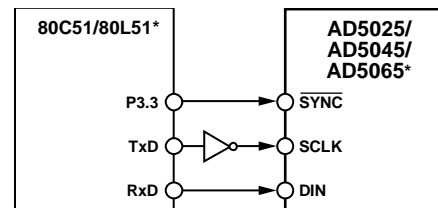
Figure 48. AD5025/AD5045/AD5065 to 80C51/80L51 Interface
