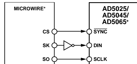
Figure 49. AD5025/AD5045/AD5065 to MICROWIRE Interface
