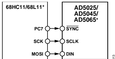
Figure 47. AD5025/AD5045/AD5065 to 68HC11/68L11 Interface
