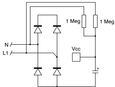
Figure 30. The full-wave connection ensures latch current continuity as well as X2-discharge path.
