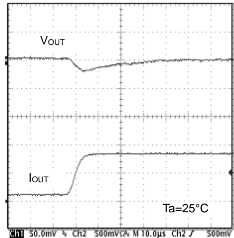
Figure 17. Transient Response (I O =125mA to 850mA, 2μA)
