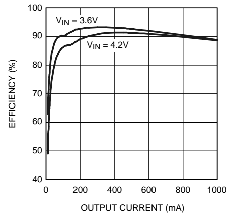
Figure 14. Efficiency vs Output Current, FPWM Mode
