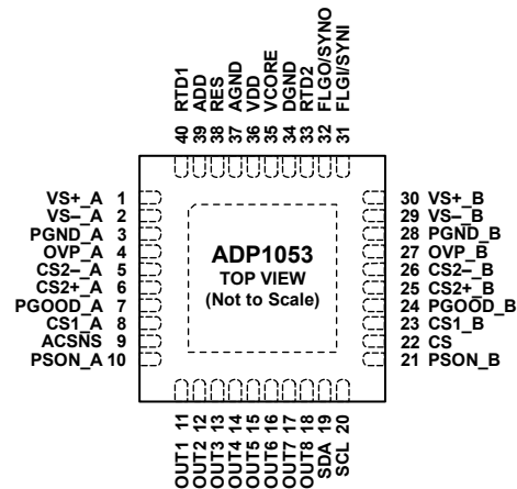
Figure 4. Pin Configuration
