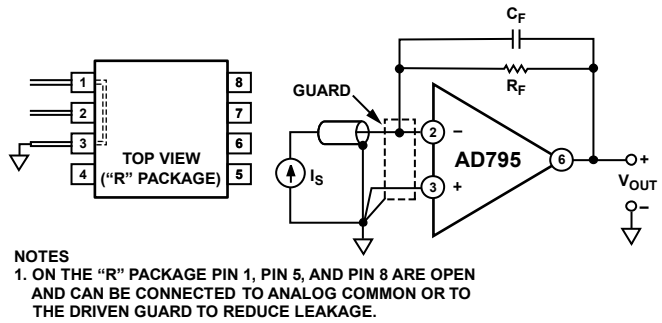
Figure 34. Guarding Scheme—Inverter
