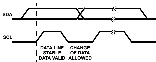
FIGURE 15. DATA VALIDITY
