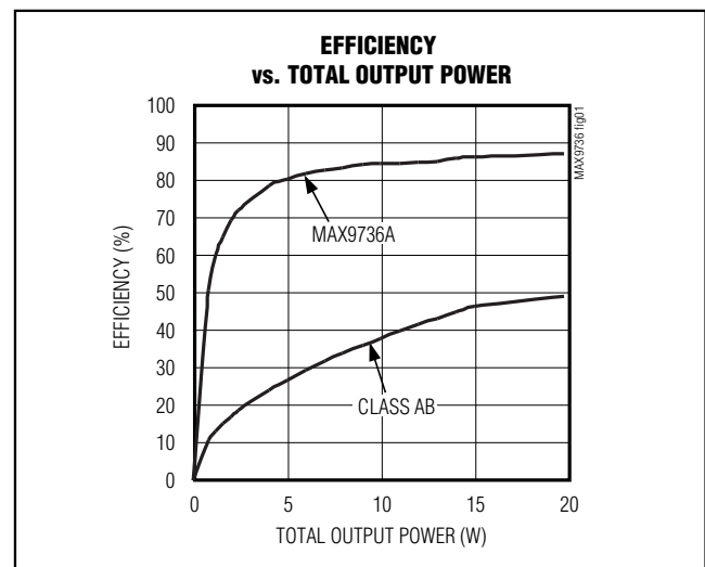
Figure 1. MAX9736A Efficiency vs. Class AB Efficiency
