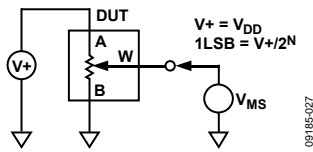
Figure 25. Resistor Position Nonlinearity Error (Rheostat Operation; R-INL, R-DNL)
