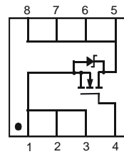
Top View Pin Configuration
