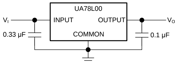
Simplified Schematic
