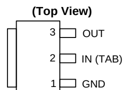
SOT223 (Fixed output) (ER Package)
