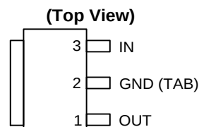
SOT223 (Fixed output) (E Package)
