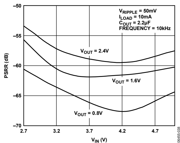
Figure 23. ADP1712 Adjustable Power Supply Rejection Ratio vs. Input Voltage
