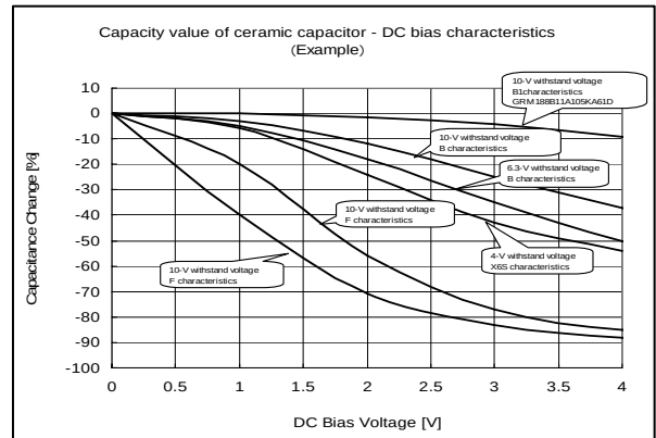
Figure 93. Capacity-bias characteristics
