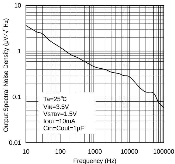
Figure 61. Output Spectral Noise Density vs. Frequency
