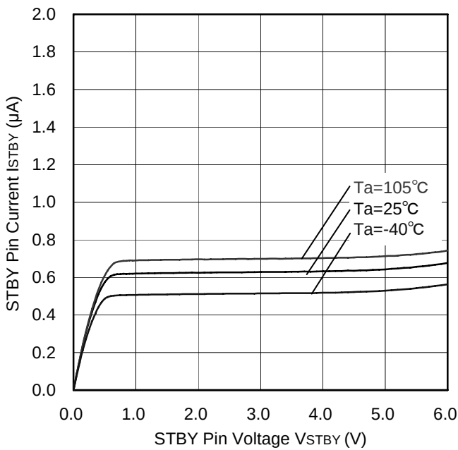
Figure 57. STBY Pin Current vs. STBY Pin Voltage
