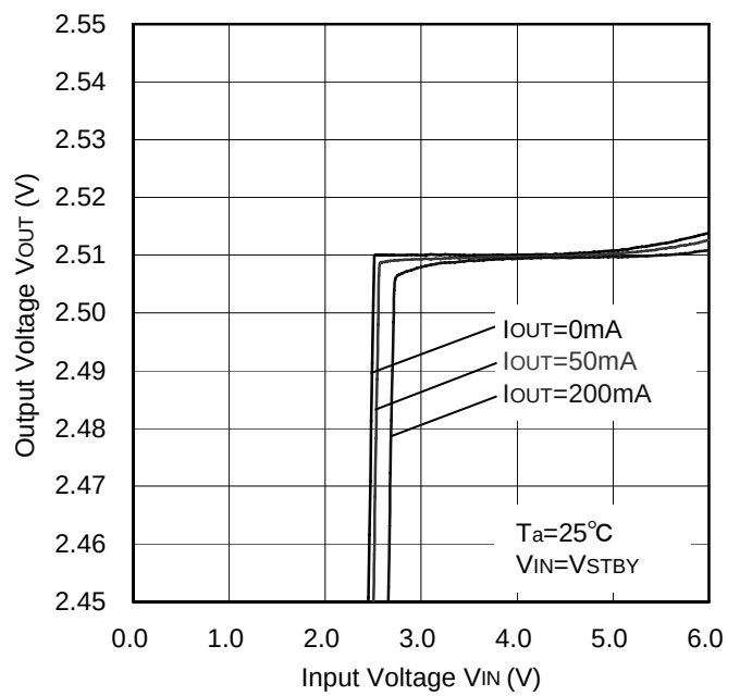
Figure 48. Line Regulation
