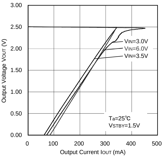
Figure 52. OCP Threshold
