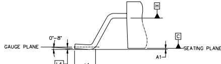
DETAIL "A" ROTATED 90° SCALE 8:1
