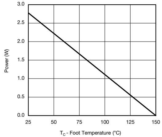
Power Derating
