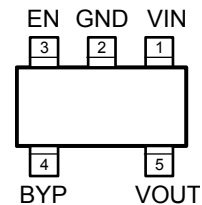
MIC5305-x.xBD5/YD5 (Fixed) TSOT-23-5 (D5) (Top View)
