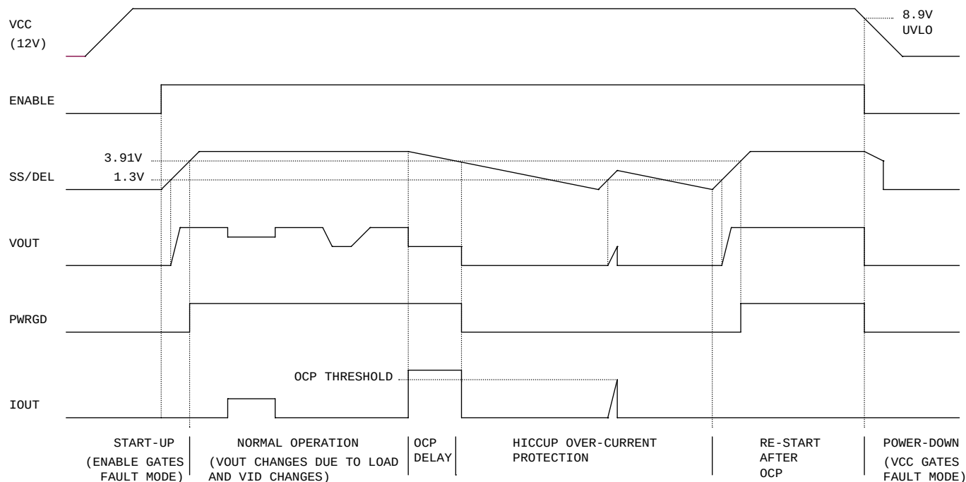
Figure 10. Operating Waveforms
