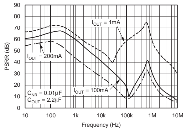
Figure 10. TPS799285 Power-Supply Ripple Rejection vs Frequency ( V_{IN} - V_{OUT} = 1.0\text{ V} )
