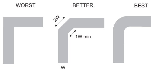
Figure 9. Trace Example
