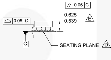
SIDE VIEWS
