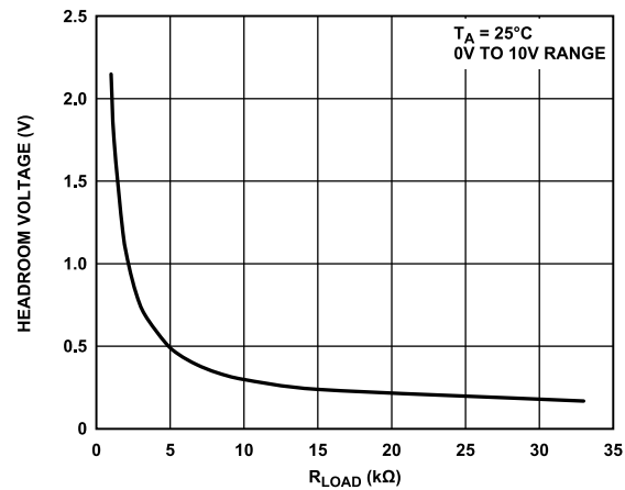
Figure 34. V_{OUT} Headroom
