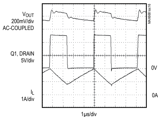
HEAVY-LOAD SWITCHING WAVEFORM
