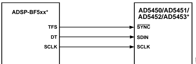
Figure 58. ADSP-BF504 to ADSP-BF592 Device Family SPORT to AD5450/AD5451/AD5452/AD5453 Interface (ADSP-BFxx Denotes the ADSP-BF504 to ADSP-BF592)
