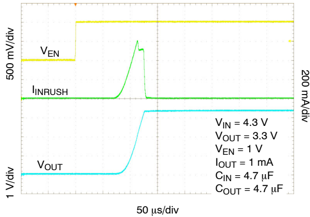
Figure 22. Enable Turn-on Response – C OUT = 4.7 μF, I OUT = 1 mA
