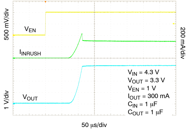
Figure 21. Enable Turn-on Response – C OUT = 1 μF, I OUT = 300 mA
