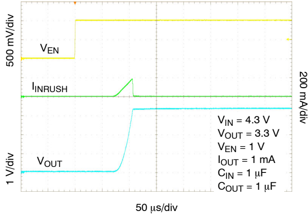
Figure 20. Enable Turn-on Response – C OUT = 1 μF, I OUT = 1 mA
