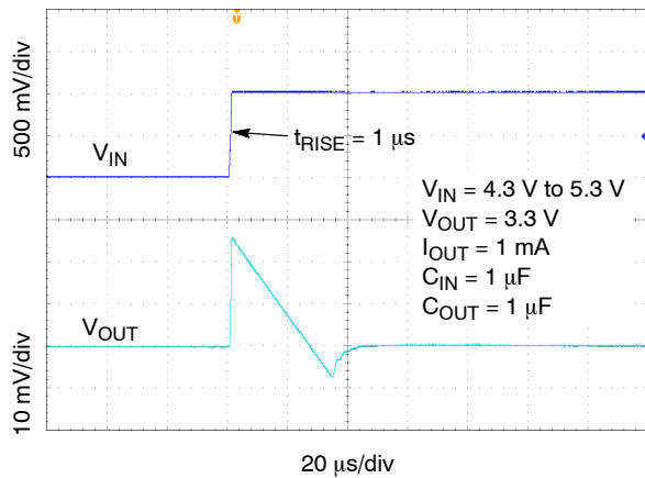
Figure 24. Line Transient Response – Rising Edge, I OUT = 1 mA
