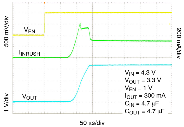
Figure 23. Enable Turn-on Response – C OUT = 4.7 μF, I OUT = 300 mA
