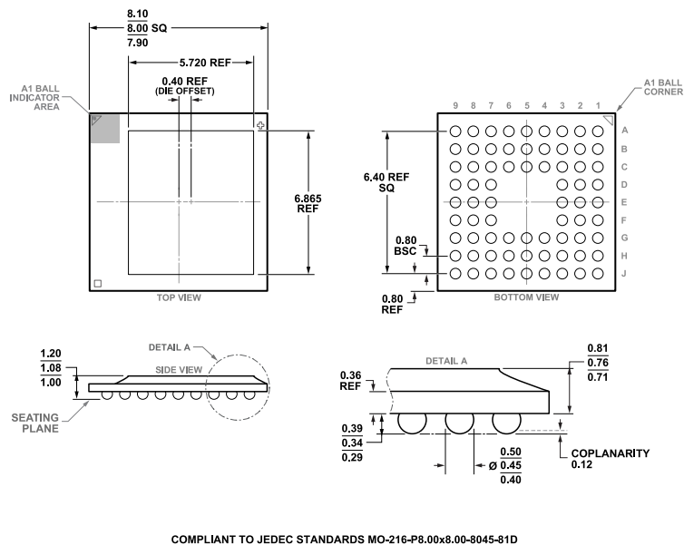
Figure 65. 72-Ball Chip Scale Package Ball Grid Array [CSP_BGA] (BC-72-2) Dimensions shown in millimeters
