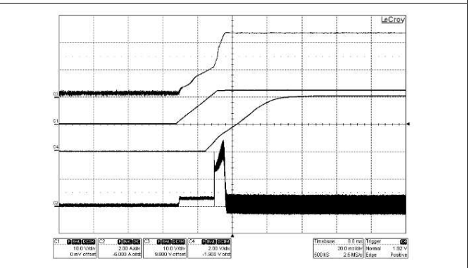
Figure 46. Skip Cycle
