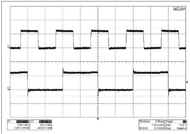
Figure 43. Clock Synchronization
