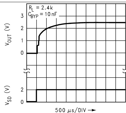
Figure 30. Turn-ON Waveform
