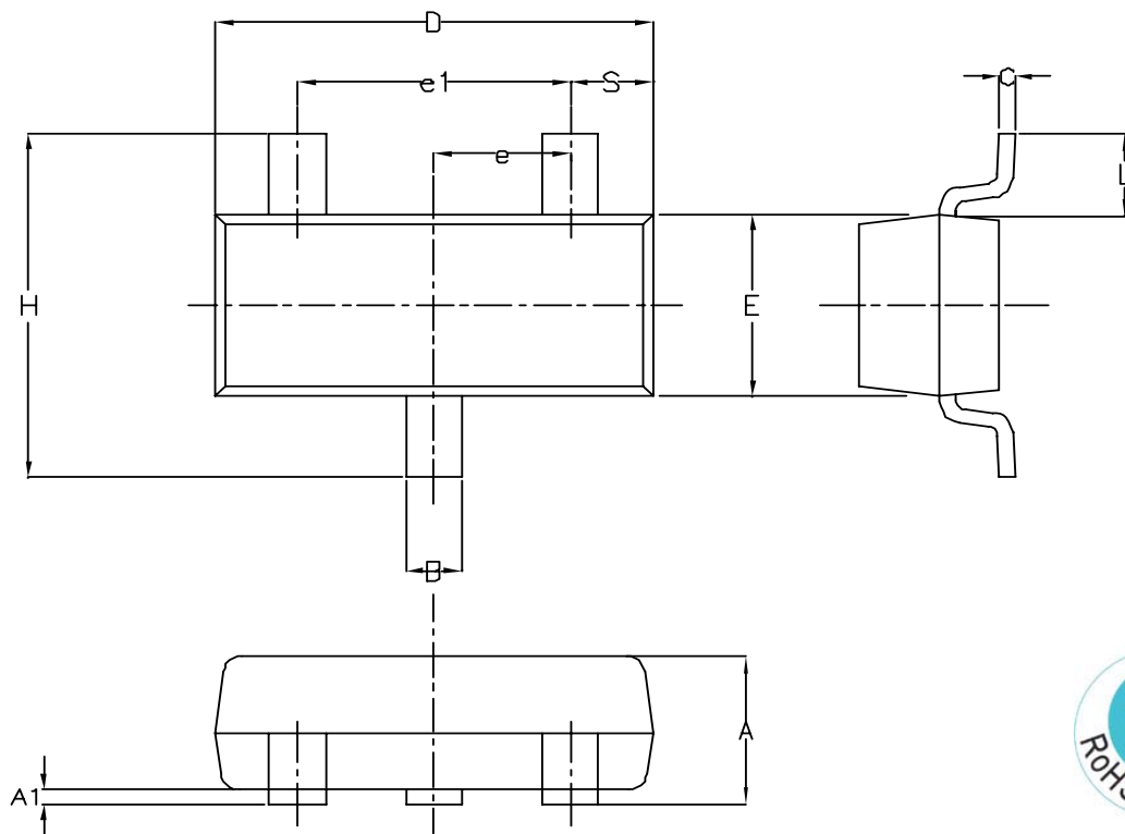
Figure 15. 3-pin SOT23 Package
