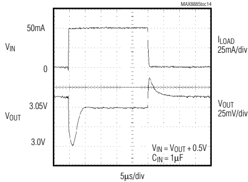
LOAD-TRANSIENT RESPONSE
