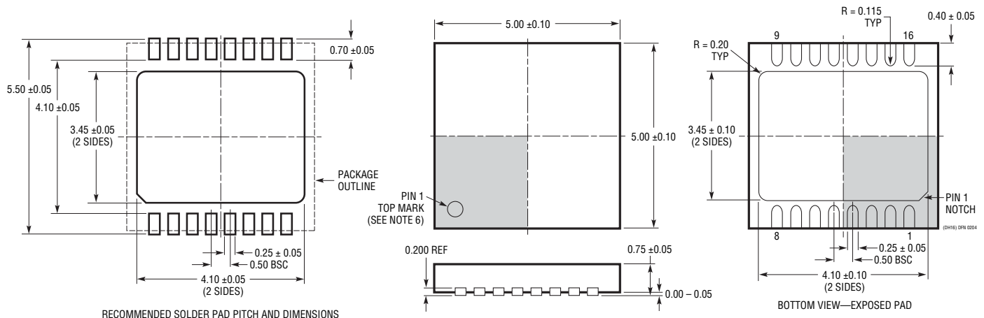
DH Package 16-Lead Plastic DFN (5mm × 5mm) (Reference LTC DWG # 05-08-1709)
