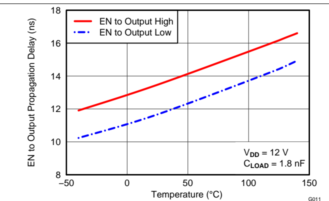
Figure 14. En to Output Propagation Delay vs Temperature
