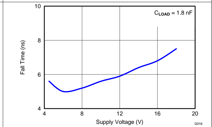
Figure 18. Fall Time vs Supply Voltage
