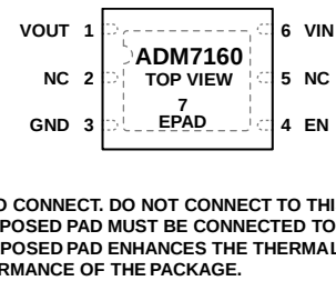
Figure 3. Pin Configuration, 6-Lead LFCSP
