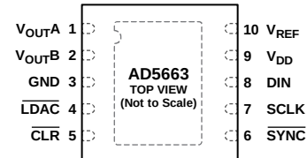
Figure 4. 10-Lead LFCSP Pin Configuration
