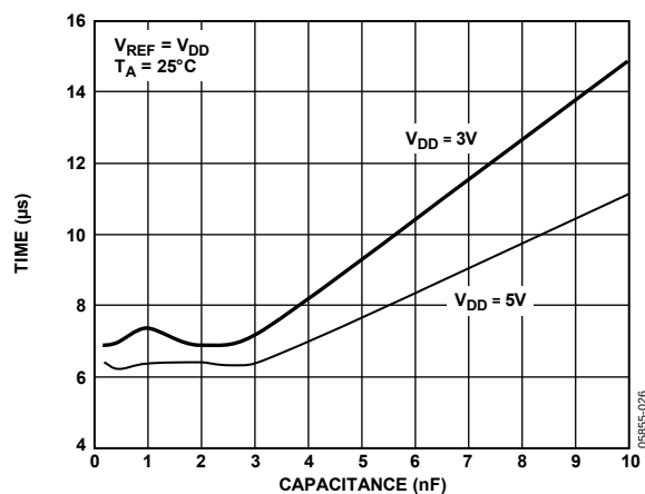
Figure 23. Settling Time vs. Capacitive Load
