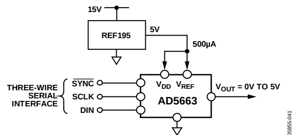
Figure 37. REF195 as Power Supply to the AD5663
