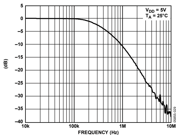
Figure 26. Multiplying Bandwidth
