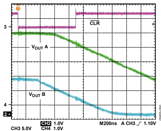
Figure 27. \overline{\text{CLR}} Pulse Activation Time
