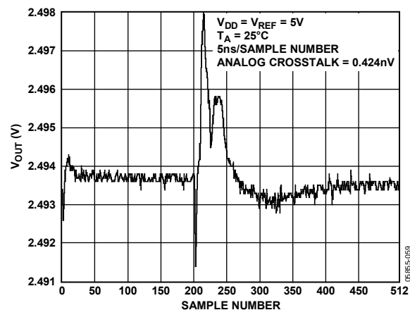
Figure 21. Analog Crosstalk
