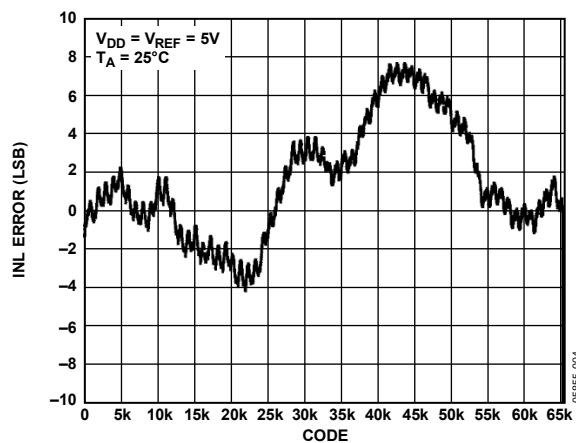
Figure 5. INL
