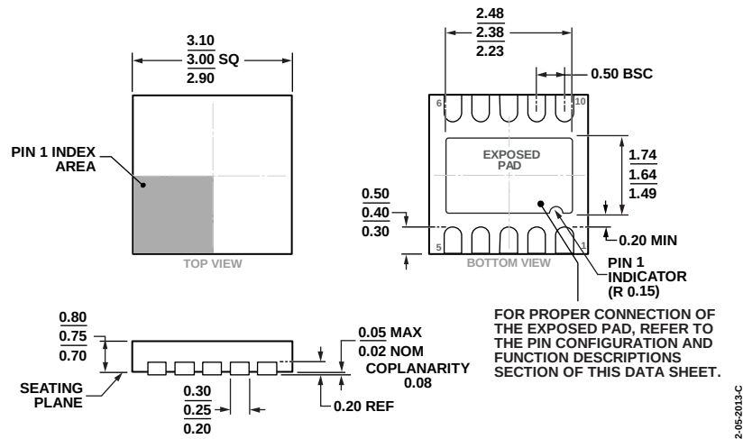
Figure 40. 10-Lead Lead Frame Chip Scale Package [LFCSP_WD] 3 mm × 3 mm Body, Very Very Thin, Dual Lead (CP-10-9)
