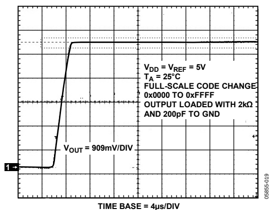
Figure 17. Full-Scale Settling Time, 5 V
