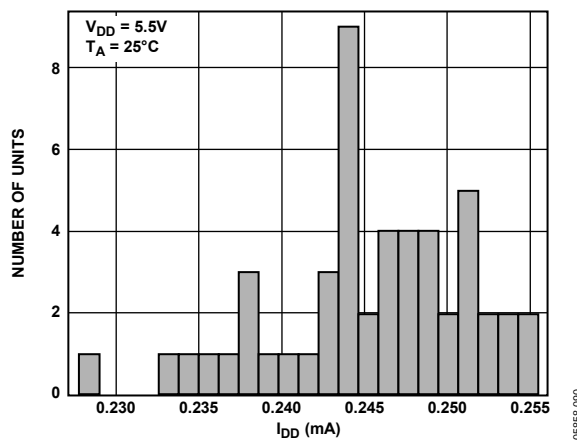
Figure 14. I_{DD} Histogram with V_{DD} = 5.5 V
