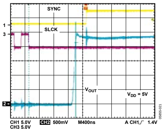
Figure 19. Exiting Power-Down to Midscale
