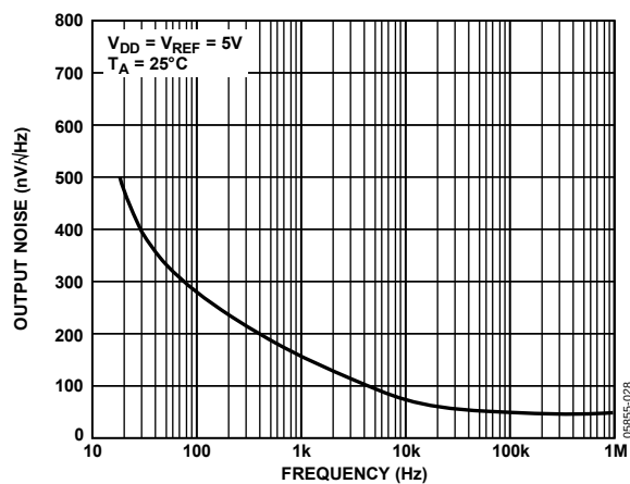
Figure 25. Noise Spectral Density
