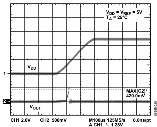
Figure 18. Power-On Reset to 0 V
