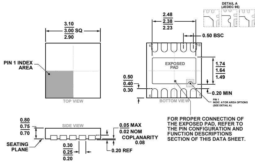
Figure 43. 10-Lead Lead Frame Chip Scale Package [LFCSP] 3 mm x 3 mm Body and 0.75 mm Package Height (CP-10-9)
