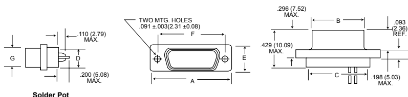
Solder Pot
