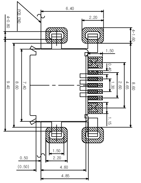
USB-IF REVERSE type Pattern USB-IF Recommended RIVERSE type Pattern (Tolerance : ±0.05)
