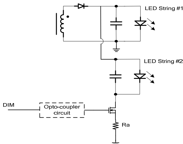
Figure 18—Color temperature and brightness control circuit
