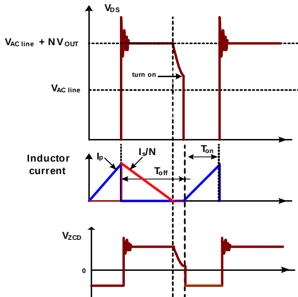
Figure 2—Boundary-conduction mode
