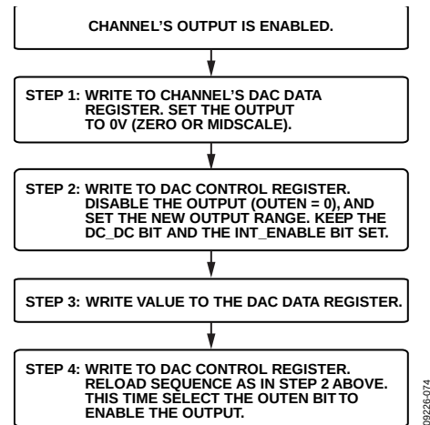
Figure 77. Steps for Changing the Output Range
