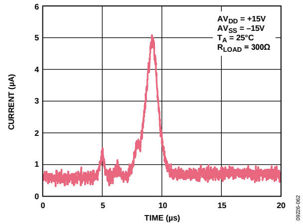
Figure 48. Output Current vs. Time on Power-Up
