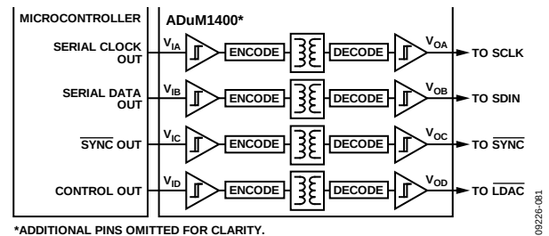
Figure 89. Isolated Interface
