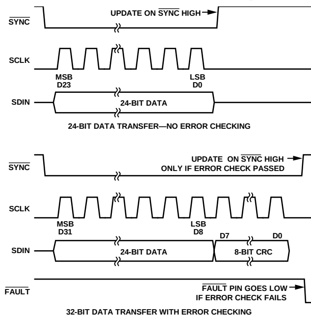
Figure 79. PEC Timing
