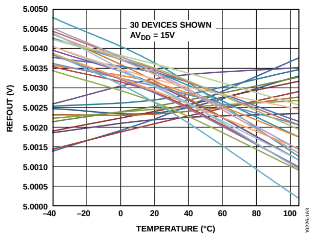
Figure 64. REFOUT vs. Temperature (When the AD5755-1 is soldered onto a PCB, the reference shifts due to thermal shock on the package. The average output voltage shift is -4\text{ mV} . Measurement of these parts after seven days shows that the outputs typically shift back 2\text{ mV} toward their initial values. This second shift is due to the relaxations of stress incurred during soldering.)
