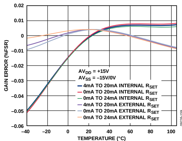
Figure 42. Gain Error vs. Temperature
