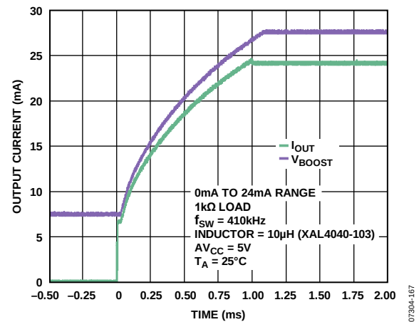
Figure 49. Output Current and V_{BOOST,x} Settling with DC-to-DC Converter (See Figure 79)
