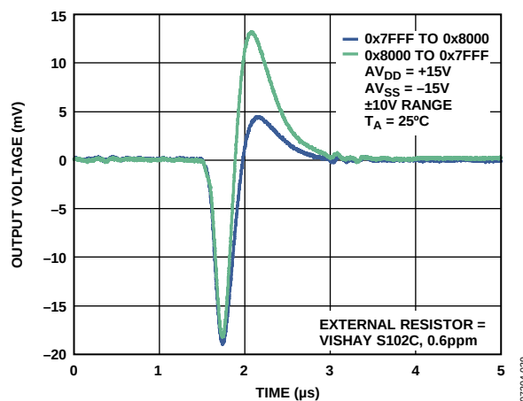
Figure 26. Digital-to-Analog Glitch
