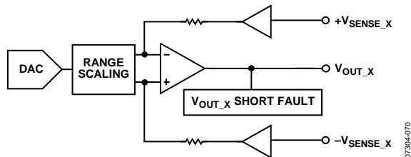
Figure 72. Voltage Output
