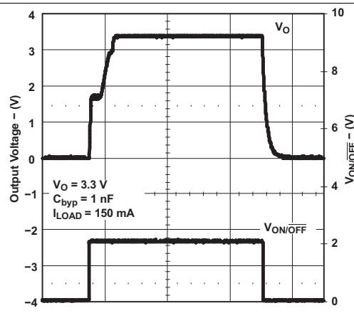
2 ms/div \rightarrow Figure 30. Turn-on Time
