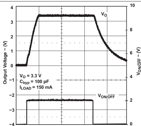
200 \mu s/div \rightarrow Figure 29. Turn-on Time
