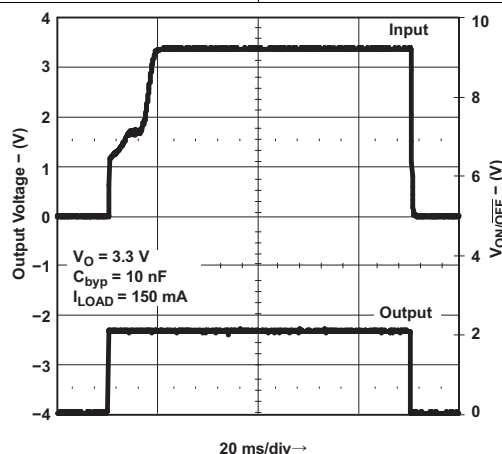
20 ms/div \rightarrow Figure 31. Turn-on Time
