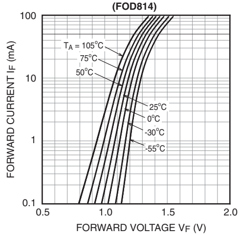
Fig. 6 Forward Current vs. Forward Voltage (FOD814)
