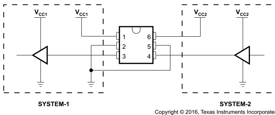
Figure 19. Unidirectional Logic Level-Shifting Application
