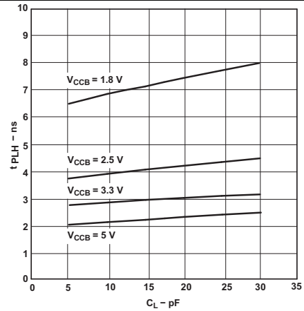
T_A = 25^\circ\text{C} , V_{CCA} = 5\text{ V} Figure 14. Typical Propagation Delay (A to B) vs Load Capacitance
