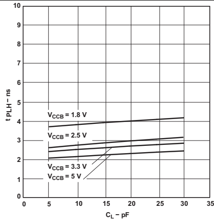
T_A = 25^\circ\text{C} , V_{CCA} = 5\text{ V} Figure 16. Typical Propagation Delay (B to A) vs Load Capacitance
