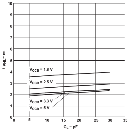
T_A = 25^\circ\text{C} , V_{CCA} = 5\text{ V} Figure 15. Typical Propagation Delay (B to A) vs Load Capacitance
