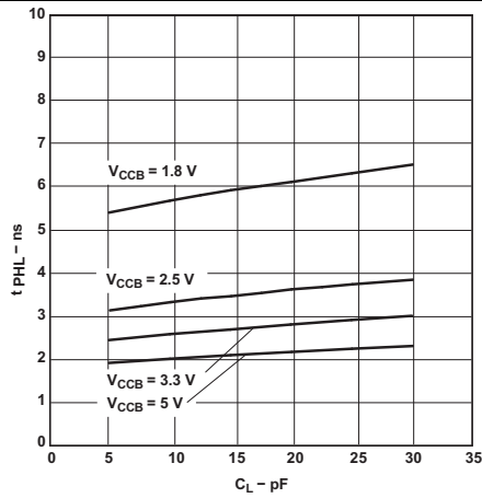
T_A = 25^\circ\text{C} , V_{CCA} = 5\text{ V} Figure 13. Typical Propagation Delay (A to B) vs Load Capacitance
