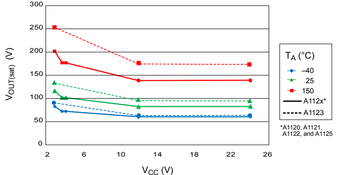
Average Output Saturation Voltage versus Supply Voltage
