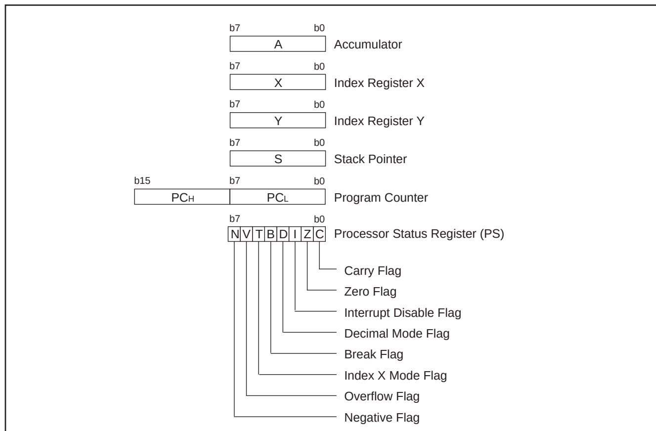
Fig. 7 740 Family CPU register structure
