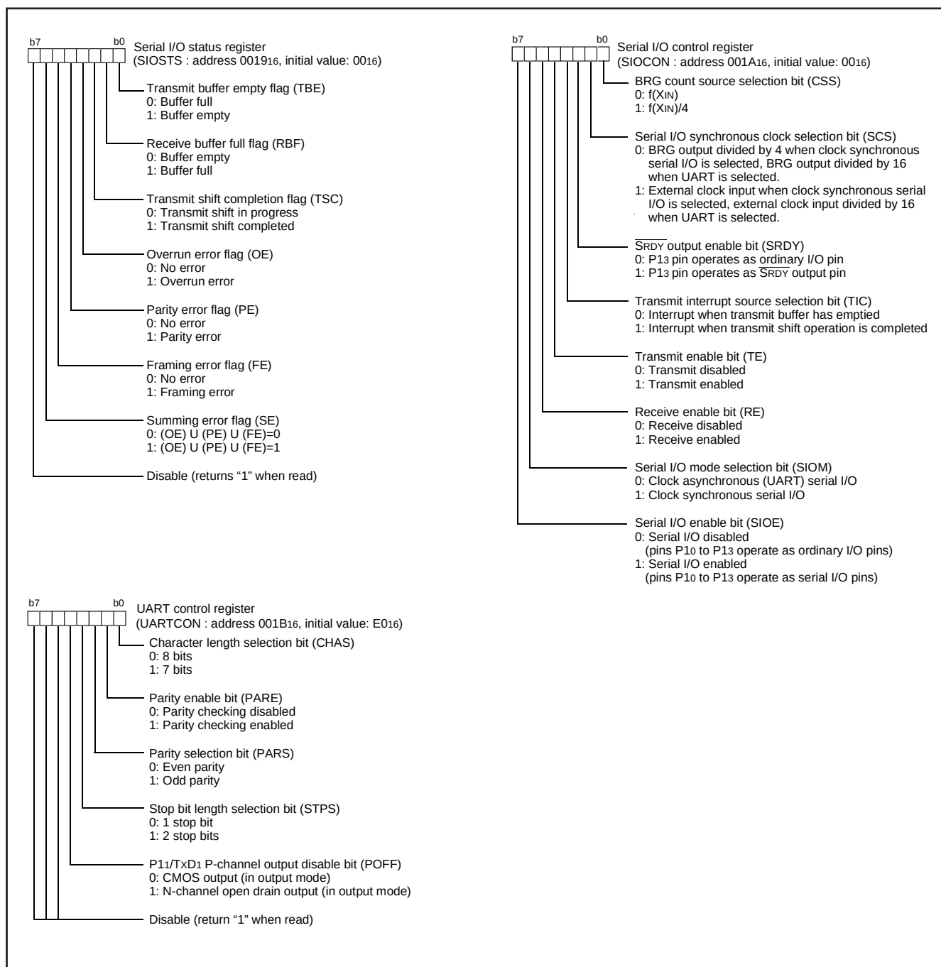
Fig. 33 Structure of serial I/O-related registers
