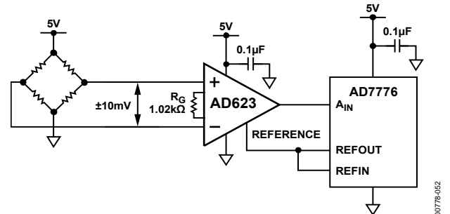
Figure 53. A Single-Supply Data Acquisition System
