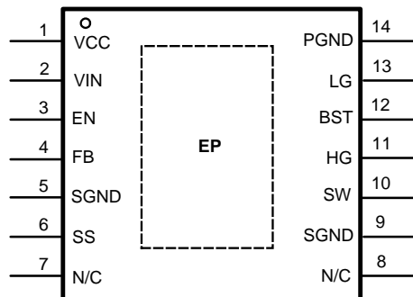
Figure 1. HTSSOP-14
