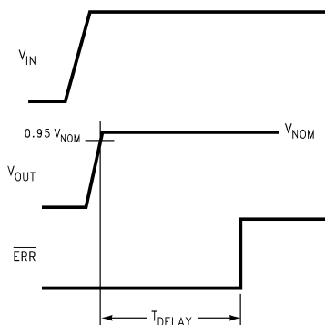
Figure 46. Timing Diagram for Power-Up
